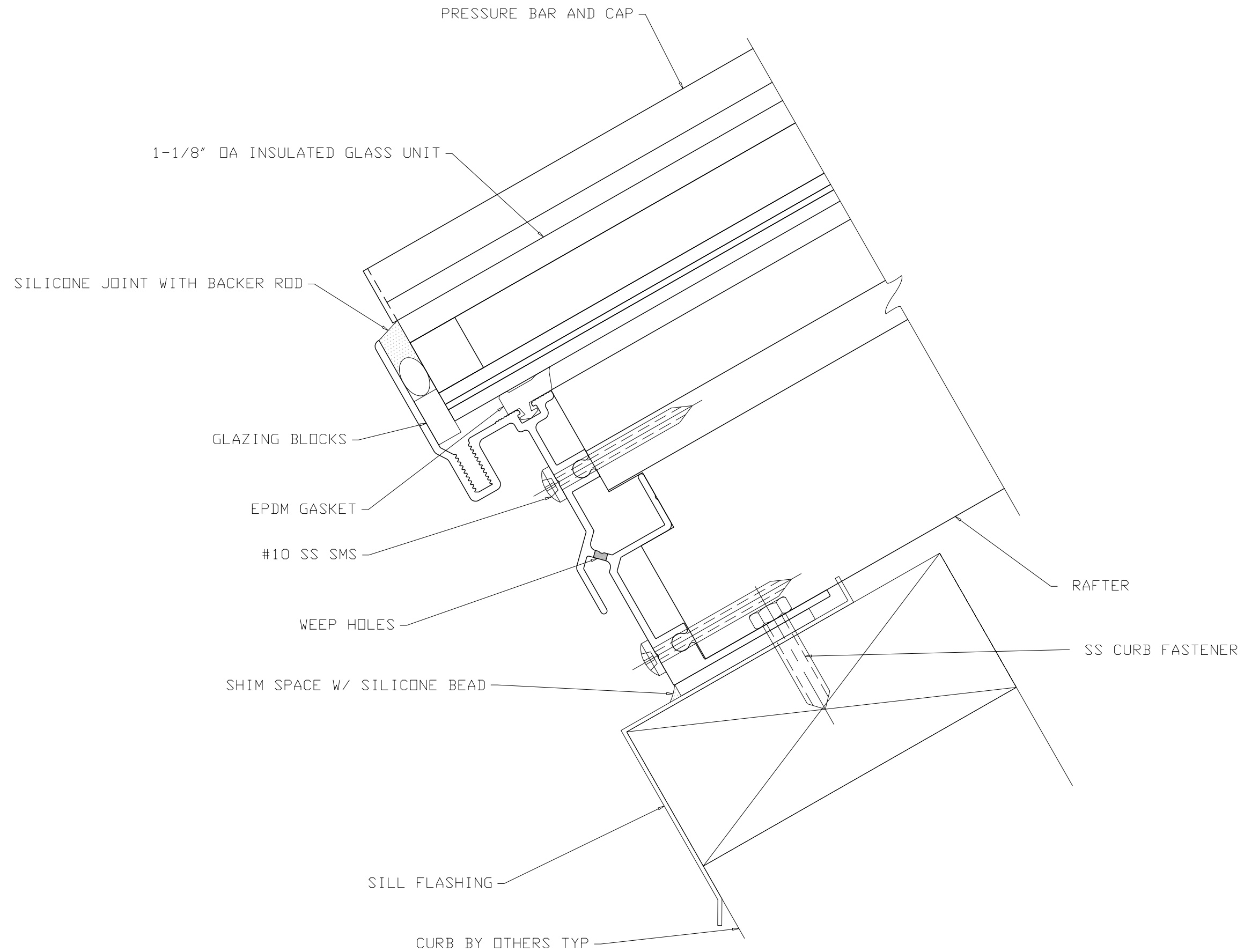
1 SILL SECTION SCALE 1' - 0" = 1' - 0"
